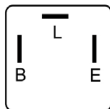
DNI1125 FLASHER 3 TERMINALES SIN SOPORTE 12V PARA: BMW, FORD, HONDA, HYUNDAI, MITSUBISHI, MAZDA, NISSAN, SUZUKI
